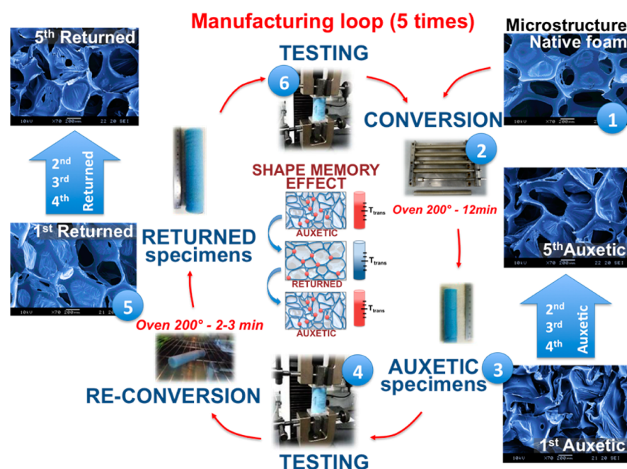
Figure 1. Multiple shape memory effect of auxetic foams. Conventional PU–PE open cell foam (1) is subjected to mechanical volumetric compression and annealing (2), obtaining a foam with negative Poisson's ratio characteristics (3). After being subjected to mechanical testing (4), the foam is placed in a oven at a temperature above the softening point, and returns to a conventional phase (5) with further testing (6). The returned-conventional foam is subjected to mechanical testing again. The conventional-auxetic-returned processing is performed five times. We obtain five auxetic phases (and five returned foam batches (1 st , 2 nd , 3 rd , 4 th , and 5 th ).
