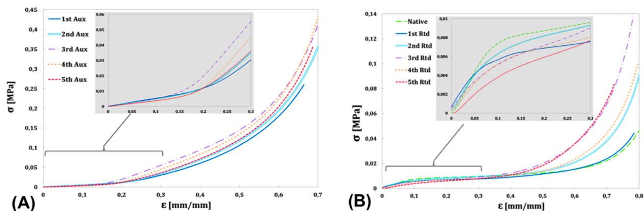
Figure 3. (a) Stress–strain compressive behavior of (a) auxetic and (b) native and returned SM foams. The auxetic specimens obtained from the 3 rd , 4 th , and 5 th SM process show a slightly higher stiffness compared to the first and second auxetic phases, because of the increase in density. The returned foams (samples belonging to the first and second phases) feature the classical linear elastic–plateau–densification compressive behavior typical of the conventional foam, although a significant hardening (more than 80% compared to the pristine phase) is present in the 2 nd and 3 rd returned foams above 60% of compressive strain. The compressive behavior of the 4 th and 5 th returned specimens is 3.7 times higher than the one of the conventional foam for the same 60% of strain.
