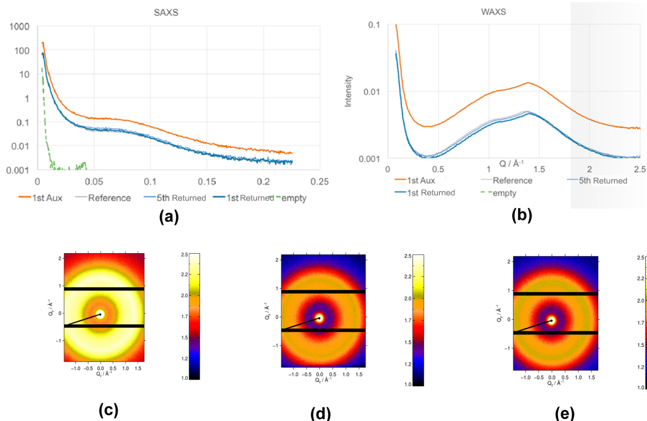
Figure 5. Logarithmic scales of the (a) SAXS scattered profiles and (b) WAXS patterns intensities for the reference foam, 1 st auxetics, 1 st returned, 5 th returned, and baseline instrument configuration. Examples of the WAXS scattered profiles are shown in (c), (d), and (e) for the 1 st auxetic, reference, and 5 th returned, respectively.
