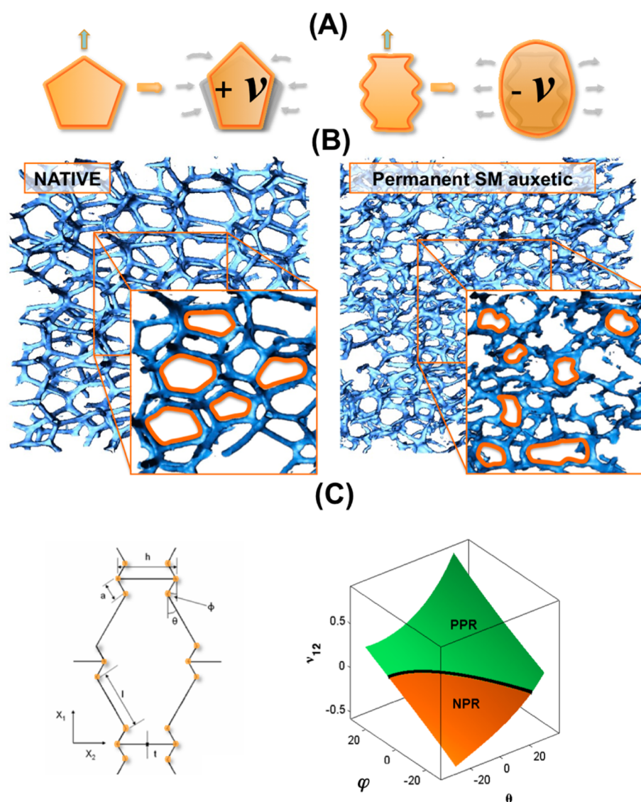
Figure 7. (a) A unit cell of conventional foam exhibiting positive Poisson's ratio ( +\nu ). A multiple re-entrant shape leads to an auxetic configuration ( -\nu ). (b) Views of \mu -CT scans of a conventional (native) and returned foam showing for the latter the multireentrant shape. (c) Idealized multireentrant cell with geometry parameters and the variation of the in-plane Poisson's ratio \nu_{12} versus the kink angles \phi and internal cell angle \theta (aspect ratio \alpha = 1.0 and kink aspect ratio \gamma = 0.5 ). 41 NPR configurations can be achieved with combinations of positive \theta and \phi angles.
